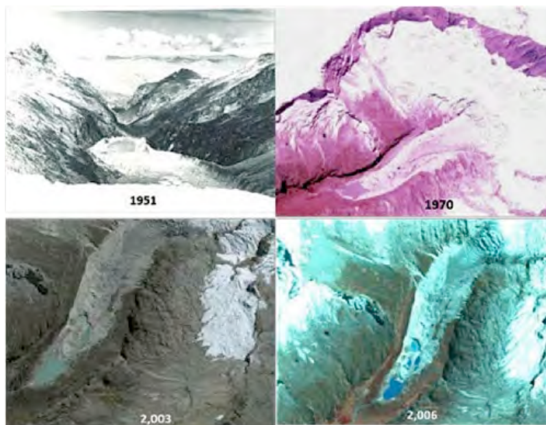
The evolution of Llacra Lake: Top row, left: 1951; right: 1970. Bottom row, left: 2003; right: 2006.
