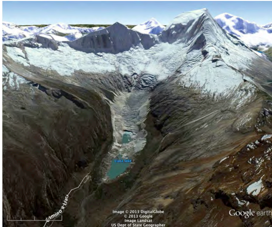
Llacra Lake showing the rapidly retreating Ranrapalca Glacier below Ranrapalca Peak (6,162 meters).
