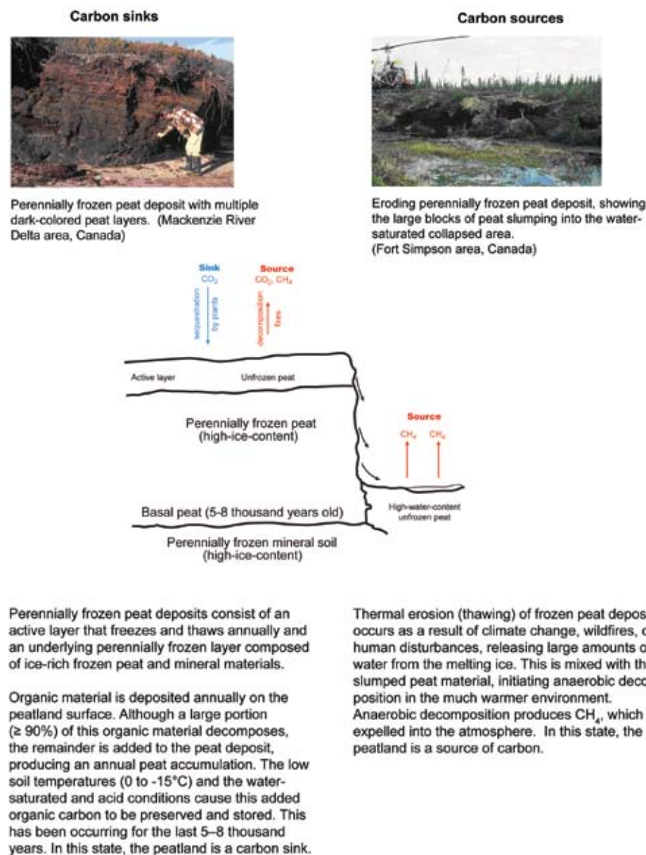
Figure 12.4 Carbon cycle in permafrost peatlands, showing below-ground organic carbon sinks and sources.
