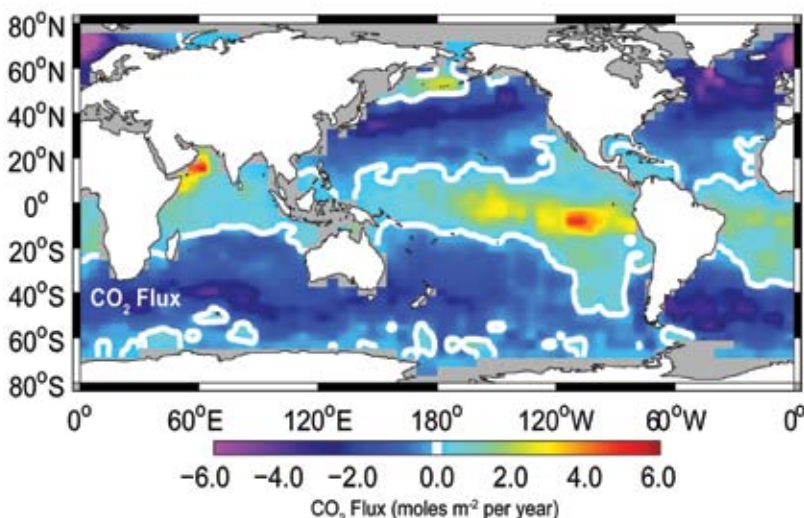
Figure 15.1 Global distribution of sea-air \text{CO}_2 flux. The source areas (cyan-green-yellow-orange) are primarily in the tropics with a few high latitude areas where deep mixing occurs in winter. The sink areas (blue-magenta) are located in mid to high latitudes. The white line represents zero flux. Updated from Takahashi et al. (2002).
