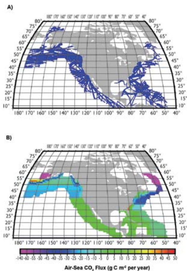
Figure 15.3 (A) Distribution of coastal surface water \text{CO}_2 partial pressure measurements made between 1979 and 2004. (B) The distribution of the annual mean air-sea net \text{CO}_2 flux over 1^\circ \times 1^\circ pixel areas (N-S 100 km, E-W 80 km) around North America. The flux ( \text{g C per m}^2 \text{ per year} ) represents the climatological mean over the 25-year period. The magenta-blue colors indicate that the ocean water is a sink for atmospheric \text{CO}_2 , and the green-yellow-orange colors indicate that the sea is a \text{CO}_2 source. The data were obtained by the authors and collaborators of this chapter and are archived at the Lamont-Doherty Earth Observatory ( www.ldeo.columbia.edu/res/pi/CO2 ).
