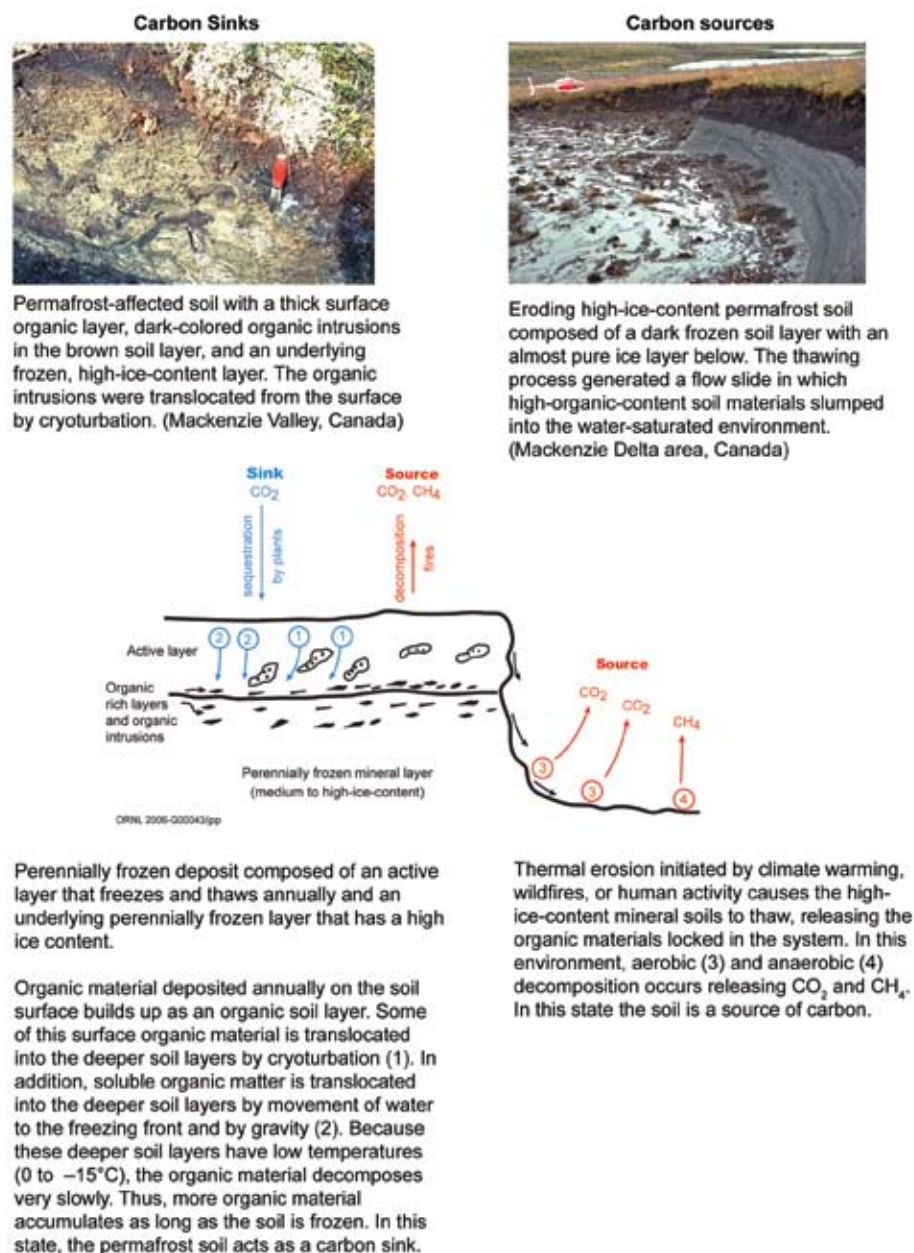
Figure 12.3 Carbon cycle in permafrost-affected upland (mineral) soils, showing below-ground organic carbon sinks and sources.
