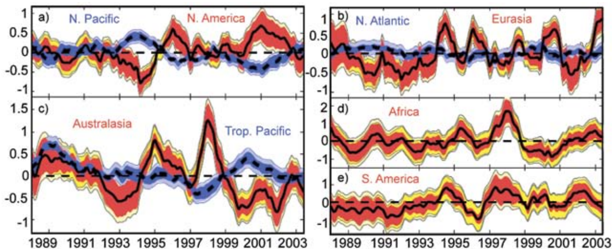
Figure 2.3 The I3-model mean CO 2 flux interannual variability (Gt C per year) for several continents (solid lines) and ocean basins (dashed lines). In each panel, the dark inner band is the 1 \sigma intermodel spread, the lighter adjacent band is the 1 \sigma estimation uncertainty on interannual variability, and the outer band (visible only for the land) is the root sum of squares of the two uncertainty components. (a) North Pacific and North America, (b) Atlantic north of 15°N and Eurasia, (c) Australasia and Tropical Pacific, (d) Africa, and (e) South America (note the different scales for Africa and South America) (Baker et al. , 2006).
