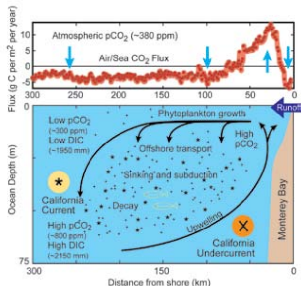
Figure 15.2 Mean air-sea \text{CO}_2 flux as calculated from shipboard measurements on a line perpendicular to the central California coast (top panel). Flux within Monterey Bay ( \sim 0 – 20 km offshore) is into the ocean, flux across the active upwelling region ( \sim 20 – 75 km offshore) is from the ocean, and flux in the California Current ( 75 – 300 km) is on average into the ocean. These fluxes result from the processes shown in the bottom panel. California Undercurrent water, which has a high \text{CO}_2 partial pressure, upwells near shore, and is advected offshore into the California Current and into Monterey Bay. Phytoplankton growing in the upwelled water use \text{CO}_2 as a carbon source, and \text{CO}_2 is drawn to low levels in those areas. Phytoplankton carbon eventually sinks or is subducted below the euphotic zone, where it decays, elevating the \text{CO}_2 levels of subsurface waters. Where the level of surface \text{CO}_2 is higher than the level of atmospheric \text{CO}_2 , diffusion drives \text{CO}_2 into the atmosphere. Conversely, where the level of surface \text{CO}_2 is lower than that of atmospheric \text{CO}_2 , diffusion drives \text{CO}_2 into the ocean. The net air-sea flux on this spatial scale is near zero. DIC = concentration of inorganic carbon (i.e., all \text{CO}_2 species) dissolved in seawater. Updated from Pennington et al. (in press).
