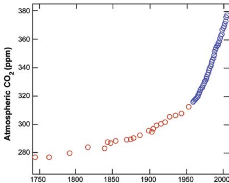
Figure 2.2 Atmospheric CO 2 concentration from 1750 to 2005. The data prior to 1957 (red circles) are from the Siple ice core (Friedli et al. , 1986). The data since 1957 (blue circles) are from continuous atmospheric sampling at the Mauna Loa Observatory (Hawaii) (Keeling et al. , 1976; Thoning et al. , 1989) (with updates available at http://cdiac.ornl.gov/trends/co2/sio-mlo.htm ).
