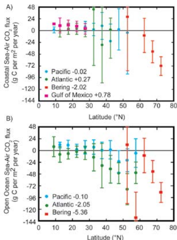
Figure 15.4 Estimated air-sea CO 2 fluxes (g C per m 2 per year) from 550,000 seawater CO 2 partial pressure (pCO 2 ) observations made from 1979 to 2004 in ocean waters surrounding the North American continent. (A) Waters within one degree (about 80 km) of the coast and (B) open ocean waters between 300 and 900 km from the shore (see Figure 15.3B). The annual mean air-sea pCO 2 difference (Δ pCO 2 ) values were calculated from the weekly mean atmospheric CO 2 concentrations in the GLOBALVIEW-CO 2 database (2004) over the same pixel area in the same week and year as the seawater pCO 2 was measured. The monthly net air-sea CO 2 flux was computed from the mean monthly wind speeds in the National Centers for Environmental Prediction/National Center for Atmospheric Research (NCEP/NCAR) database in the (wind speed) 2 formulation for the air-sea gas transfer rate by Wanninkhof (1992). The ± uncertainties represent one standard deviation.
