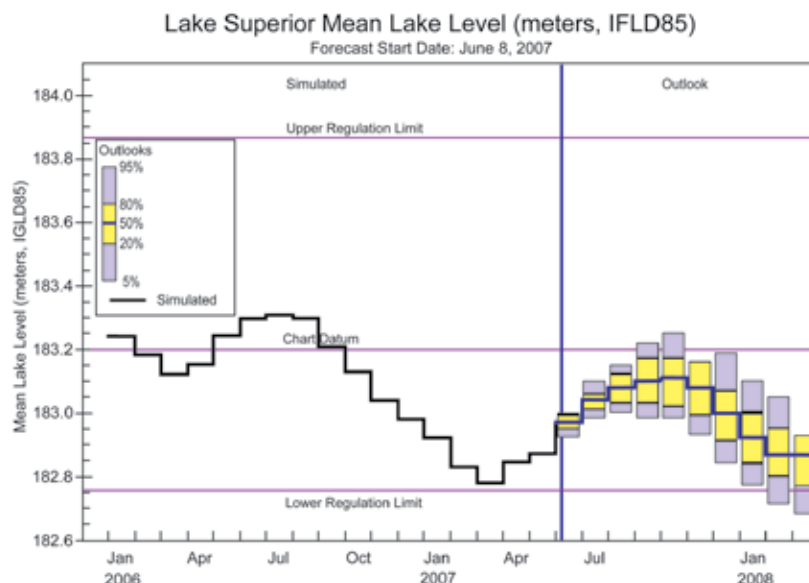
Figure 2.8 Probabilistic forecasts of future lake levels disseminated by GLERL. From: < http://www.glerl.noaa.gov/wr/ahps/curfscst/ >.
