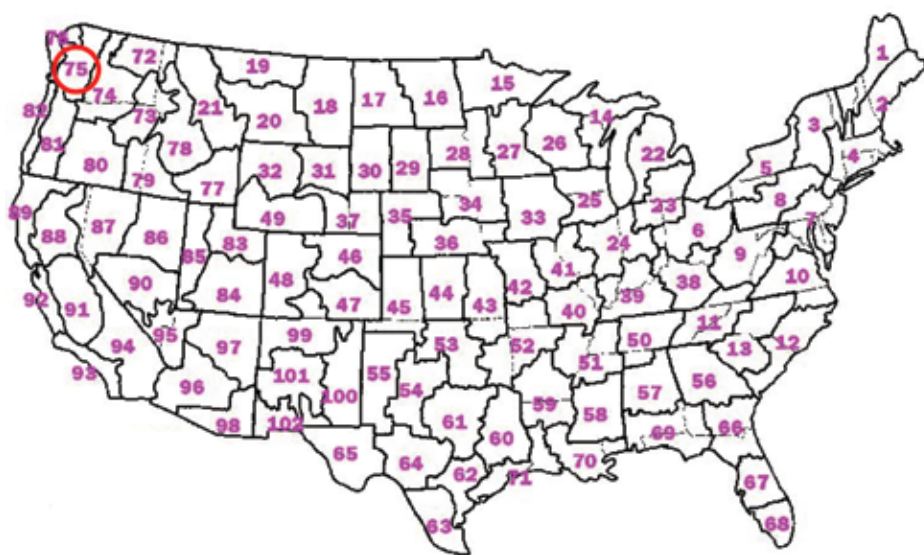
Figure 2.19 The CPC climate division spatial unit upon which the official seasonal forecasts are based. Figure obtained from < http://www.cpc.ncep.noaa.gov/products/predictions/long_range/poe_index.php?lead=3&var=p >.
