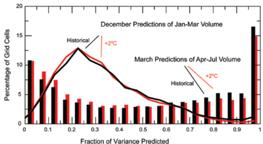
Figure 2.15 Distributions of overall fractions of variance predicted, in Figure 2.13, of January to March (curves) and April to July (histograms) runoff volumes under historical (black) and +2^{\circ}\text{C} warmer conditions (Dettinger, 2007).
