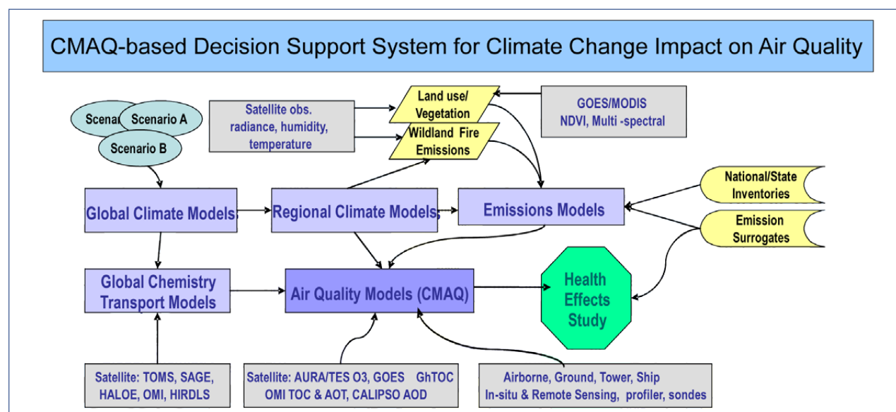
Figure 2-1 Configuration of CMAQ-based DST for Climate Change Impact Study
