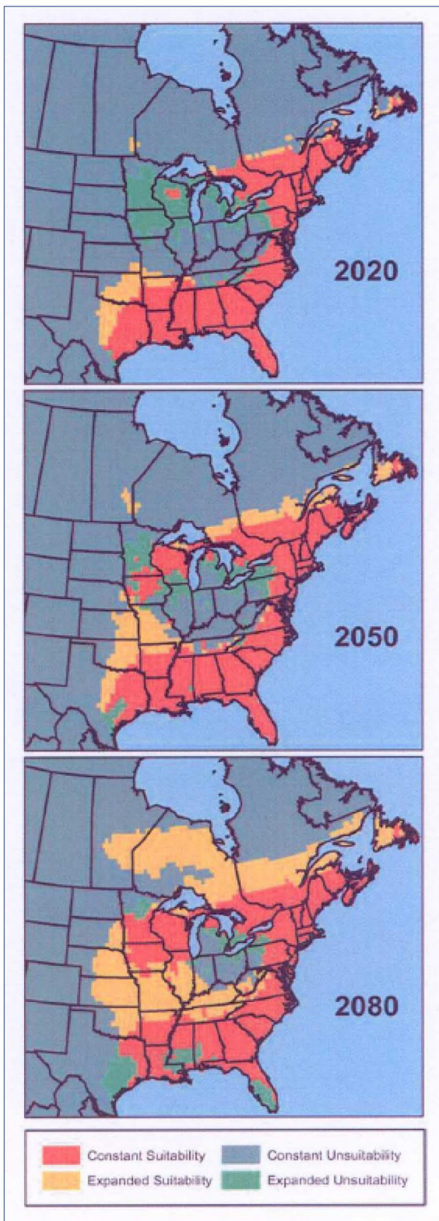
Figure 4-3 Forecast change in black-legged tick distribution in eastern and central North America under climate change scenarios using DSSPL (Brownstein et al., 2005a, EcoHealth)
