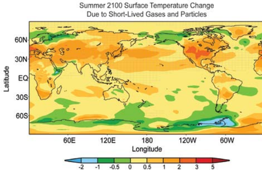
Figure 3.10 Surface temperature change in °C due to short-lived gases and particles during Northern Hemisphere summer for 2100 to 2091 vs. 2010 to 2001 in the GFDL model.
