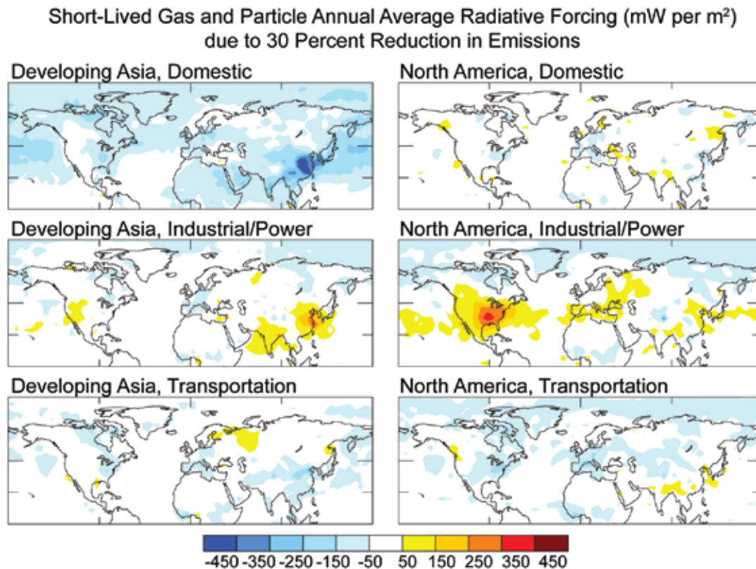
Figure 3.13 Short-lived gas and particle annual average radiative forcing (mW per m 2 ) due to 30 percent reductions in emissions from the given region and economic sector in the GISS model.
