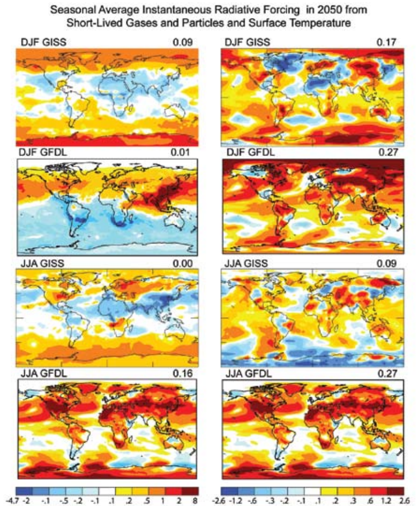
Figure 3.8 Seasonal average instantaneous radiative forcing ( \text{W per m}^2 ) in 2050 from short-lived gases and particles (left column) and surface temperature response in ^{\circ}\text{C} (right column) in the GISS and GFDL models. Boreal winter (December through February) is shown in the top two rows, while boreal summer (June through August) is shown in the bottom two rows. The temperature changes at 2050 are 2046 to 2055 in the GFDL model and 2041 to 2050 in the GISS model. Values in the upper right corners give the global mean. (Note that the instantaneous forcings shown here for the GFDL model differ from the adjusted forcings show in Table 3.6.)
