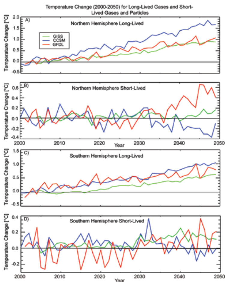
Figure 3.6 Hemispheric mean annual average temperature change (°C) in the simulations with time-varying long-lived and short-lived gases and particles. All the results are three-member ensemble means for GFDL and GISS and single member simulations for CCSM. Results for the short-lived gases and particles are obtained by subtraction of the (long-lived) calculations from the (short+long-lived) calculations.
