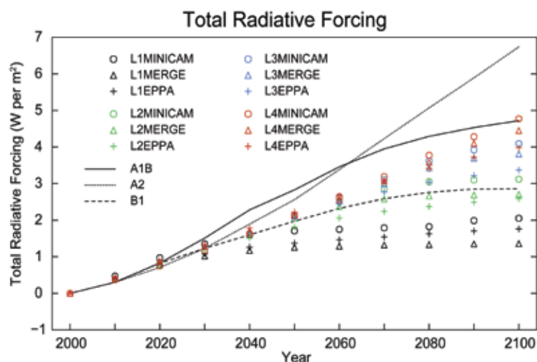
Figure 2.3 Total radiative forcing ( \text{W per m}^2 ) calculated by MAGICC for the 12 SAP 2.1a scenarios (Clarke et al. , 2007) plotted with the total calculated by MAGICC for the B1, A1B, and A2 scenarios (IPCC, 2001).
